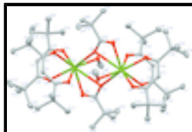
Fig. 1. The molecular structure of the title complex, with the numbering scheme and displacement ellipsoids drawn at the 35% probability level [the H atoms have been omitted for clarity].
